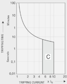
Tripping characteristic C
